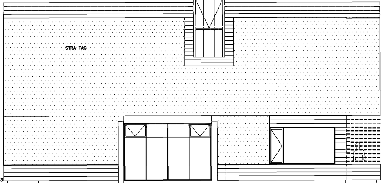
FACADE VEST
